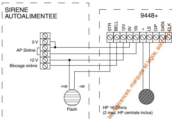
Figure 18. Raccordement sirène
